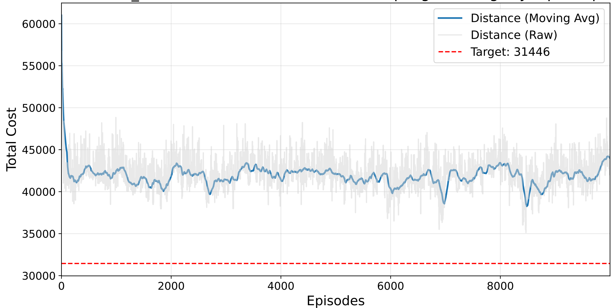
Final NO_MASK Masked AutoRL-SOP (Resampling) Training - ry48p.4.sop
